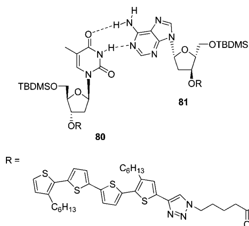
Figure 13. Structures of adenosine-quaterthiophene 81 and the corresponding thymidine 80 .
