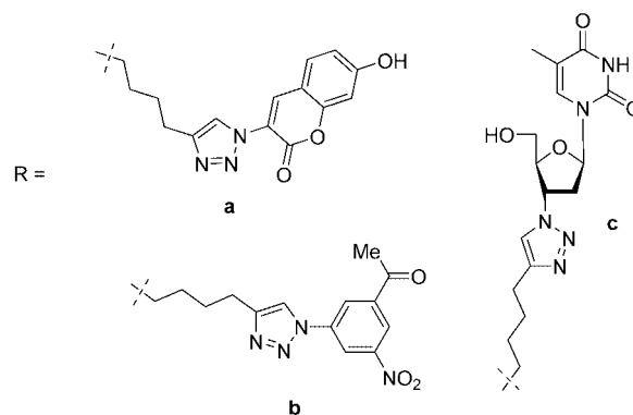
Figure 9. Structures of nucleoside conjugates 57 – 59 .
