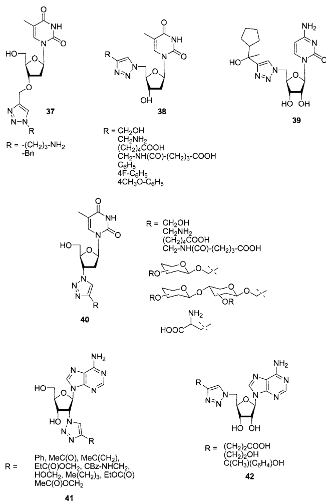
Figure 5. Structures of compounds 37–42.
